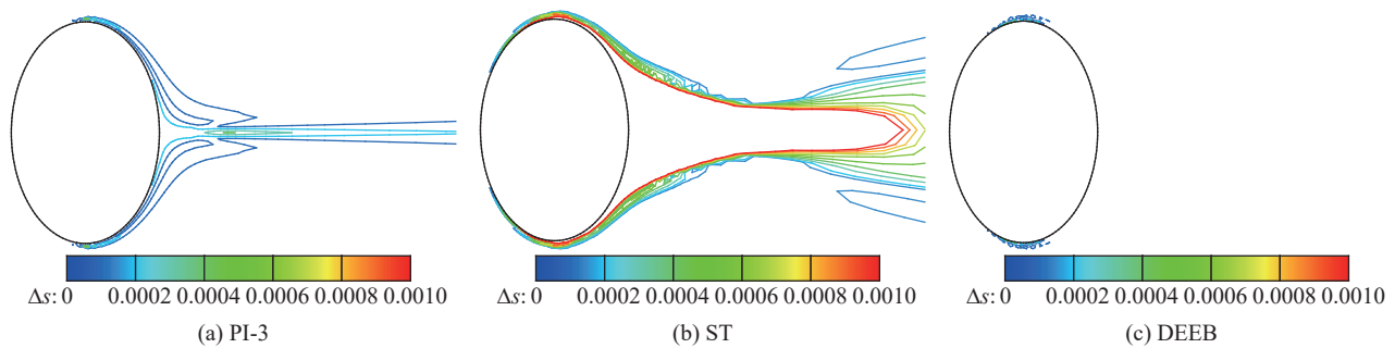
图 20 椭圆后缘绕流熵增等值线 Fig. 20 Entropy contours around the elliptic
