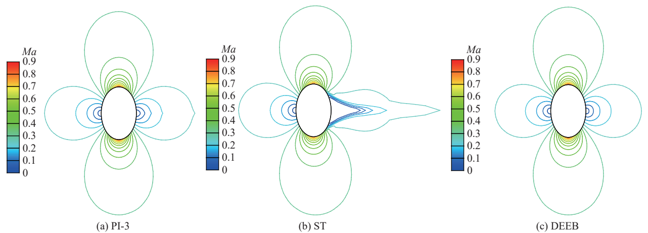
图 18 椭圆绕流马赫数等值线 Fig. 18 Mach number contours around an elliptic
